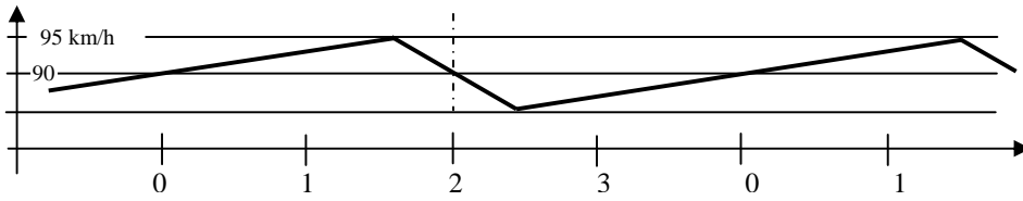
Figure 15 Circling offset from the centre of a thermal, speed at outflow.
