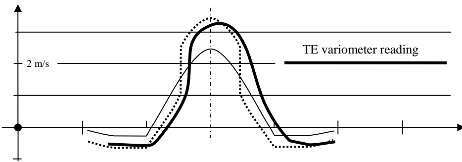
Figure 14 Distribution of the vertical flow and TE variometer reading at inflow.
