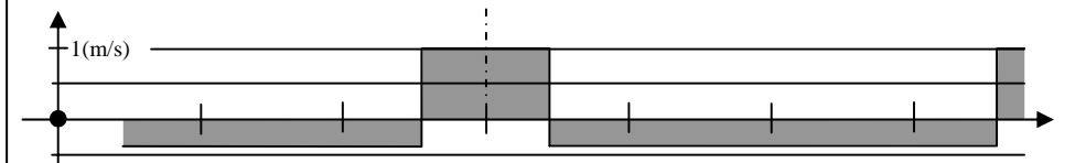
Figure 13 Additional TE variometer signal at inflow.
